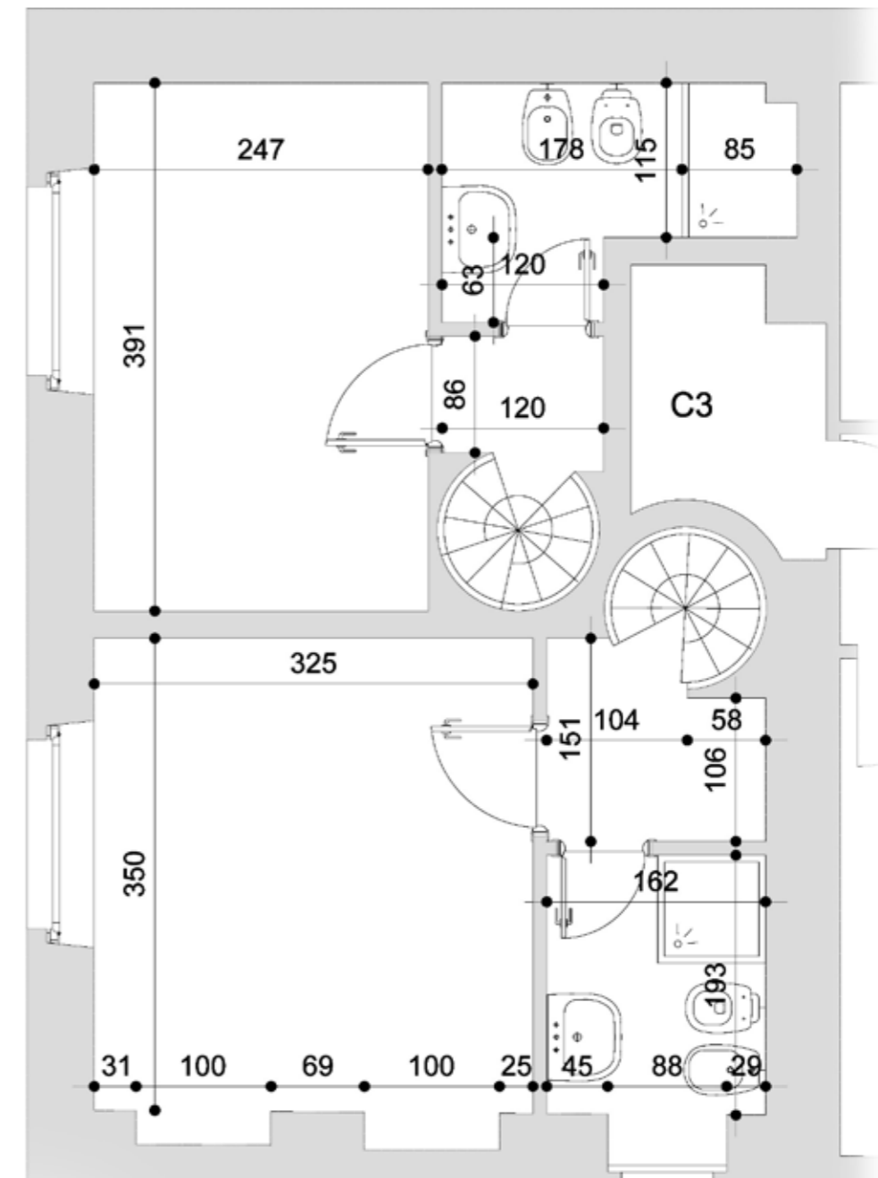
PIANO SEMINTERRATO
